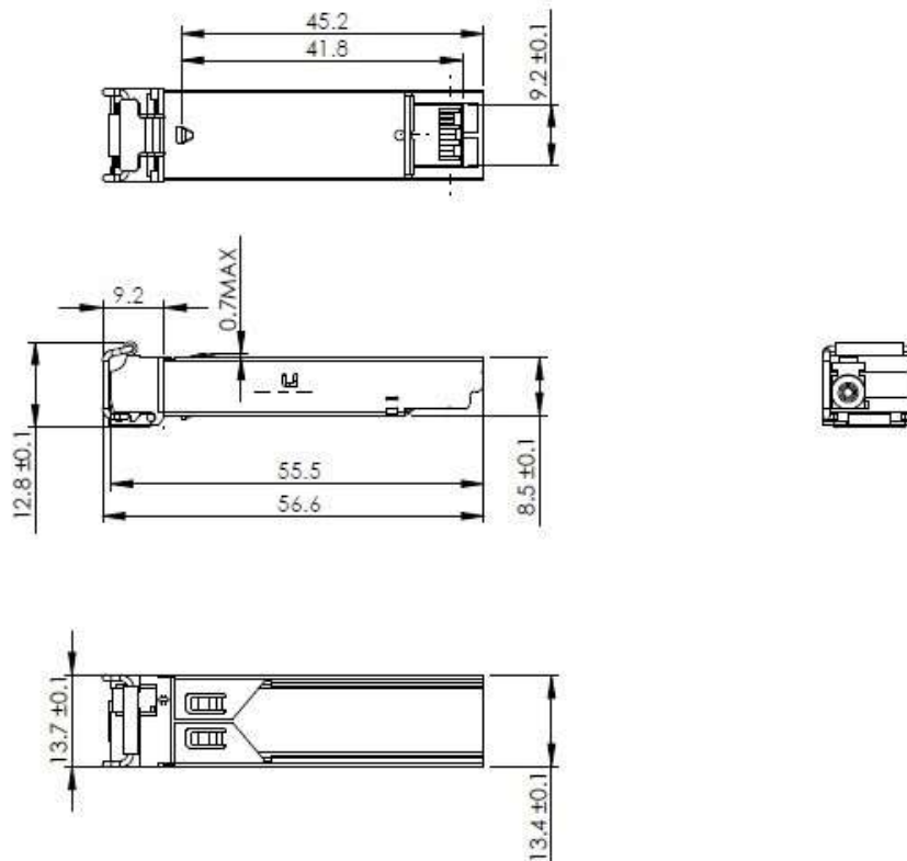
Mechanical Drawing
