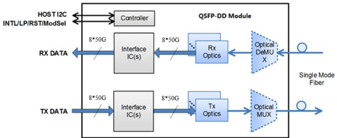
Figure 1-1 Transceiver block diagram
