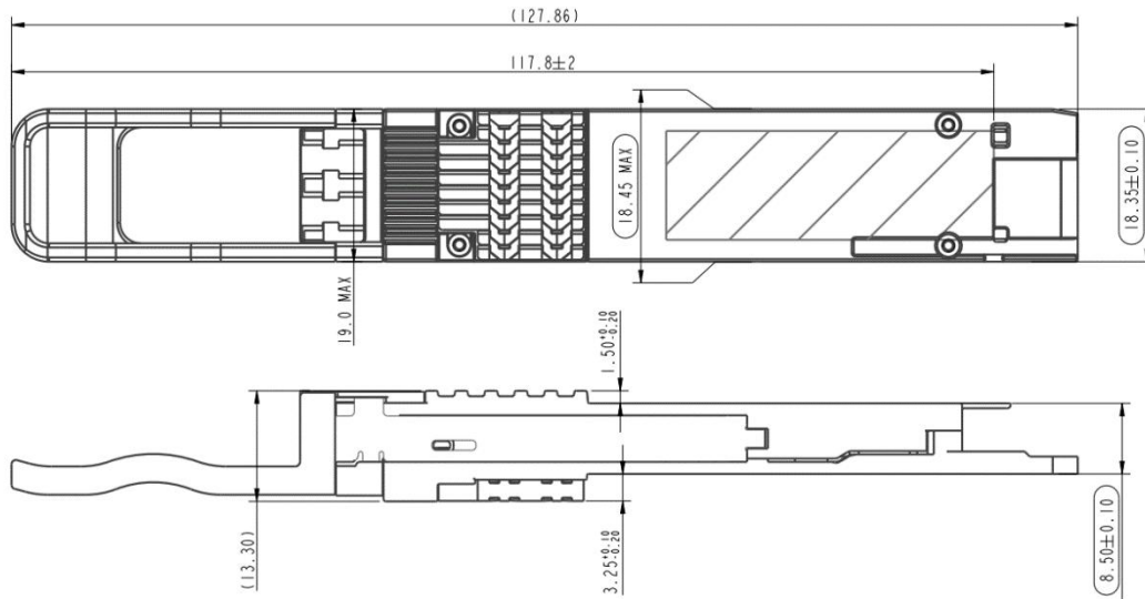
Figure 10-1 Mechanical dimensions
